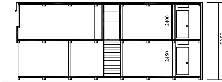
SECTION A
