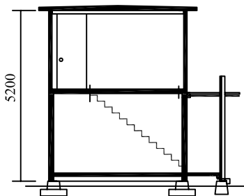
SECTION B
