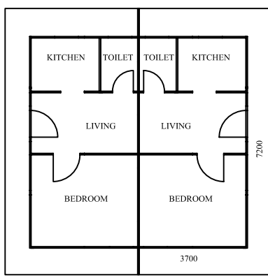
PLAN 1
