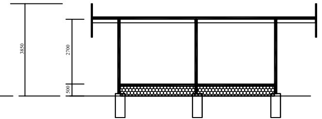
SECTION B
