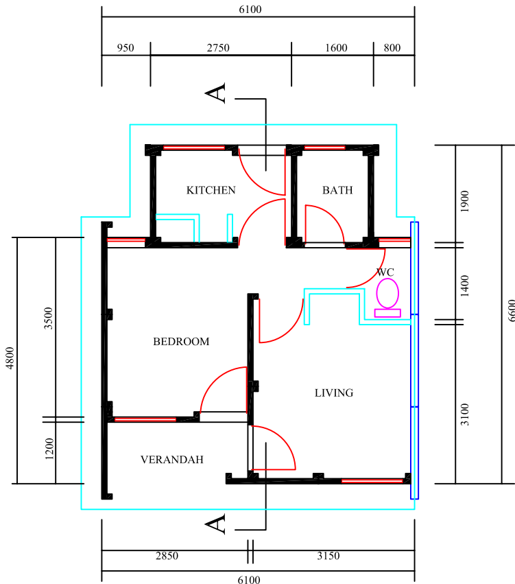
PLAN
