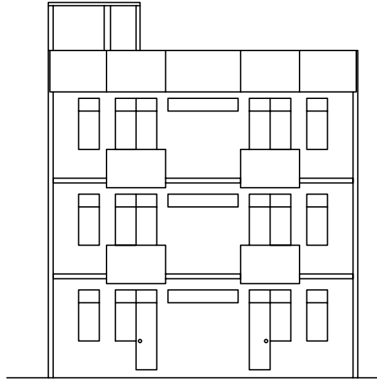
REAR ELEVATION
