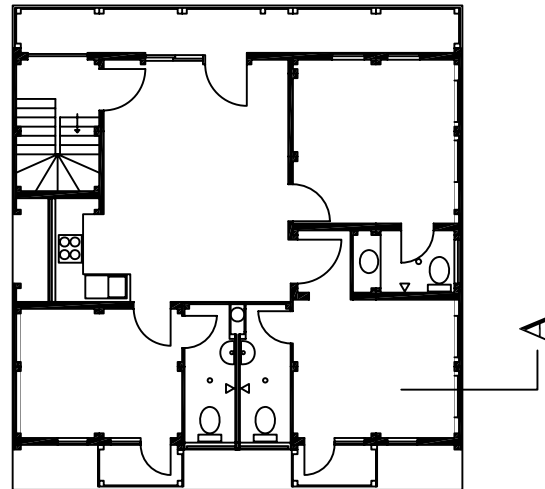
FLOORS 1 & 2
