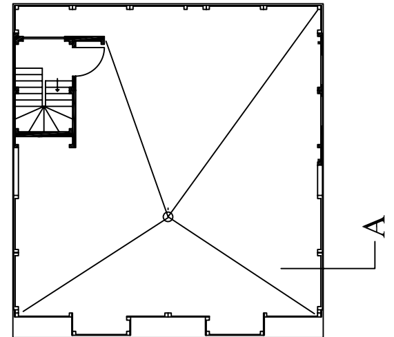
ROOF
