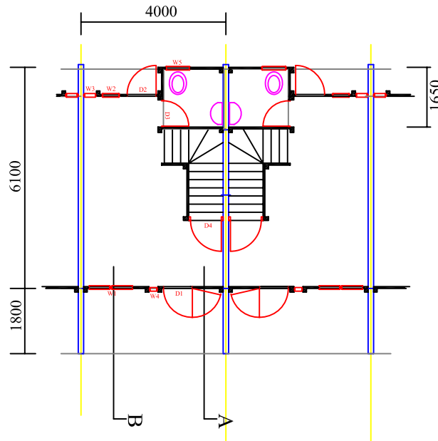
PLAN - LOWER
