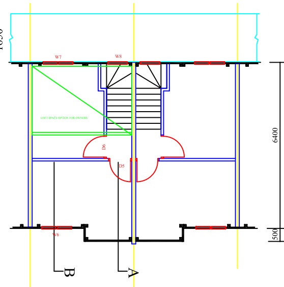
PLAN - UPPER
