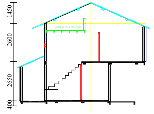
SECTION A
