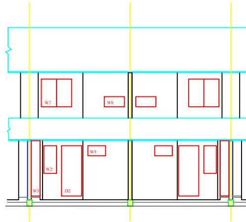
REAR ELEVATION
