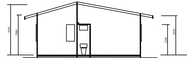
SECTION C
