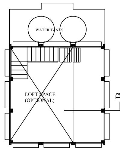
FIRST FLOOR (LOFT SPACE ABOVE)
