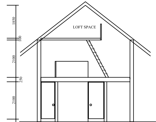
SECTION B (LOFT OPTIONAL)
