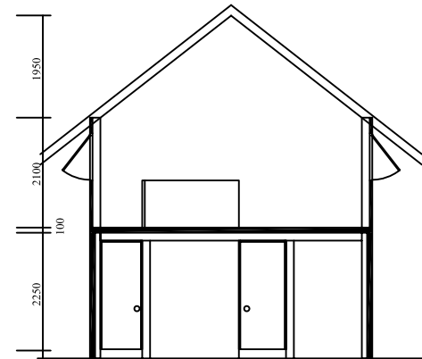
SECTION A
