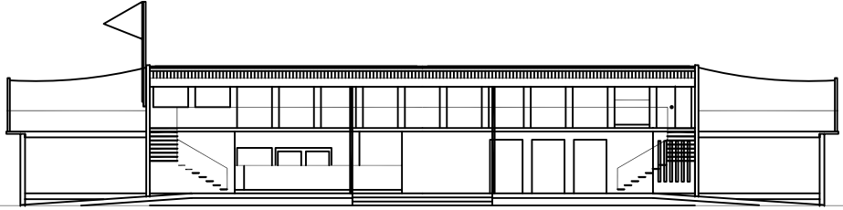
FRONT ELEVATION
