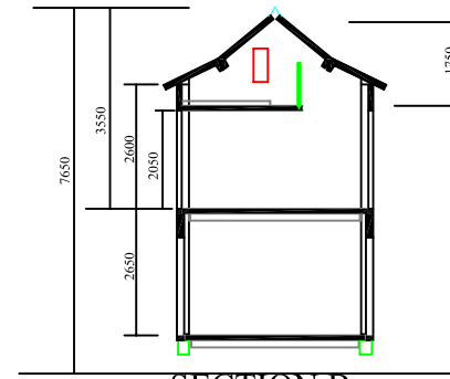
SECTION B
