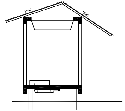
SECTION C
