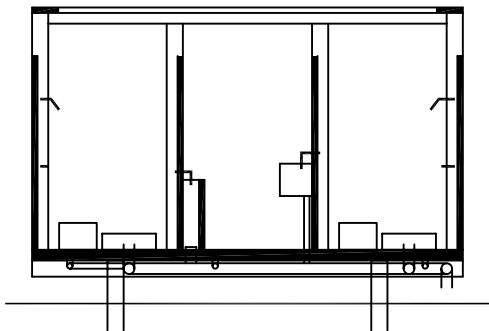
SECTION A
