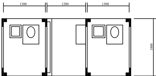
SECTION B
