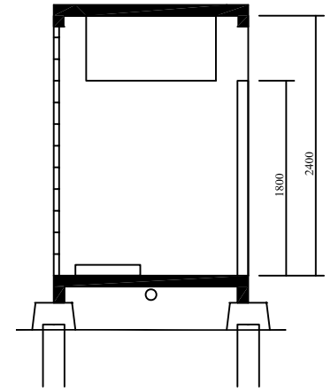
SECTION A
