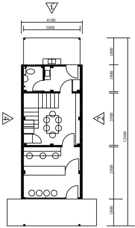
PLAN GROUND FLOOR
