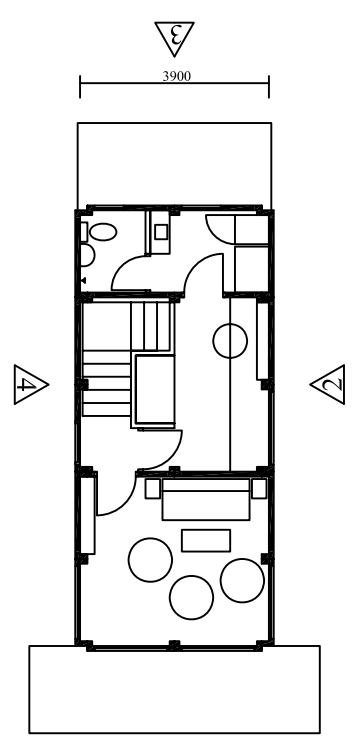
PLAN TOP FLOOR
