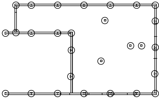
FOOTINGS
