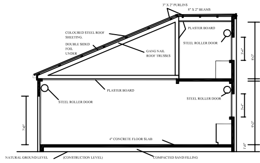
SECTION B
