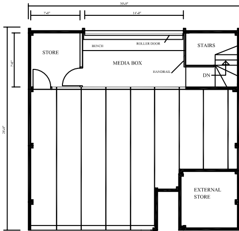
2ND FLOOR
