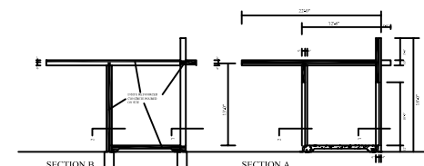
PRECAST PANELS
