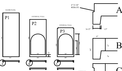
PRECAST PANELS
