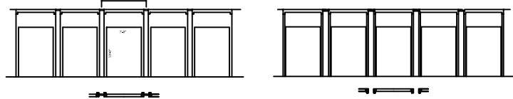
STREET ELEVATION
