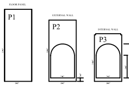
PRECAST PANELS
