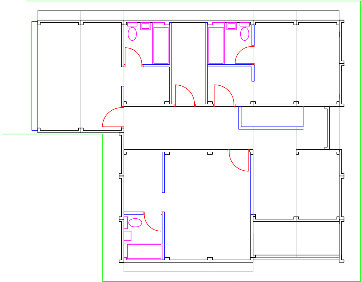
UPPER FLOOR
