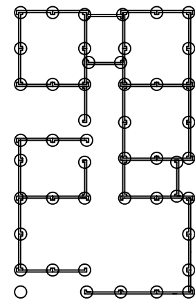
STRUCTURE - FOOTINGS
