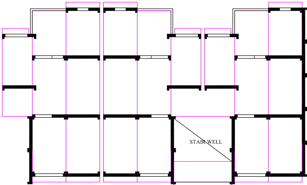
PRECAST WALL & FLOOR COMPONENTS
