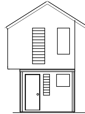
REAR ELEVATION
