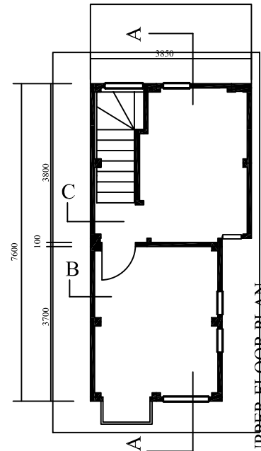
LOWER FLOOR PLAN
