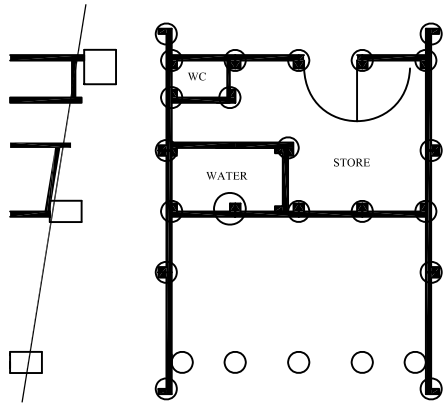
FOUNDATIONS
