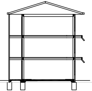
SECTION C
