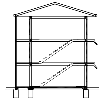
SECTION D
