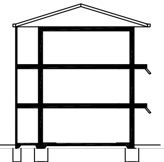
SECTION E
