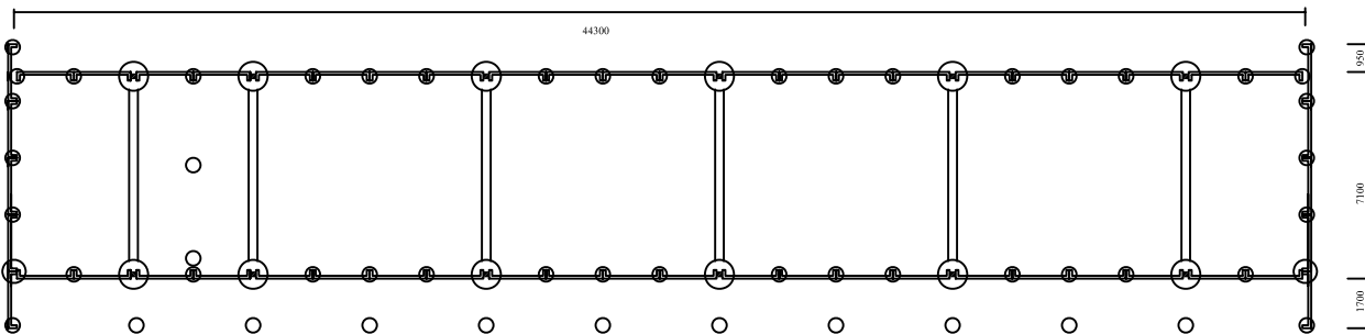
FOUNDATION PLAN
