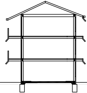
SECTION C
