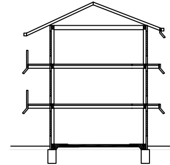
SECTION B
