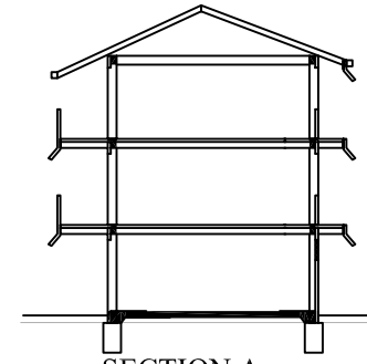
SECTION A
