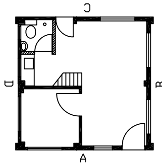
PLAN - FULL HOUSE - COMPLETE
