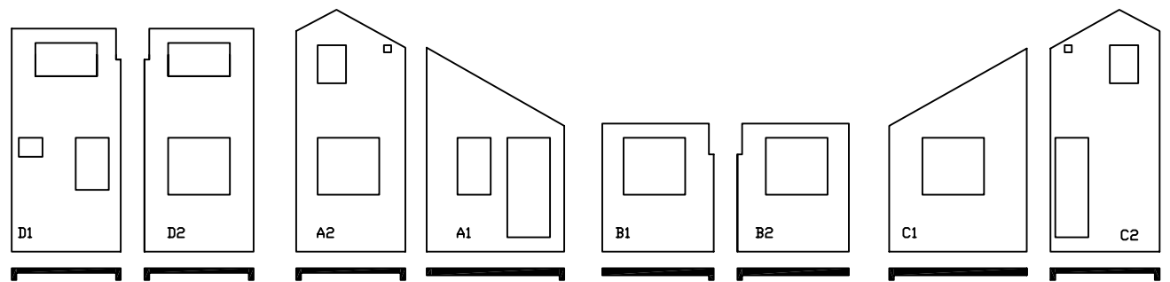
PRECAST WALLS - STARTER HOME
