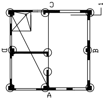
PLAN - FULL HOUSE - STRUCTURE
