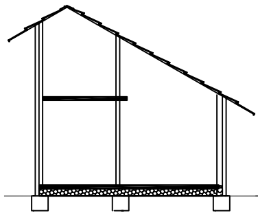
SECTION 1
