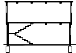
STAIR PROFILE
