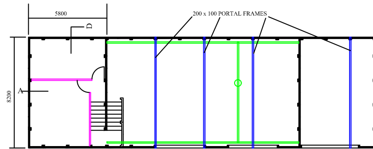
UPPER FLOOR PLAN
