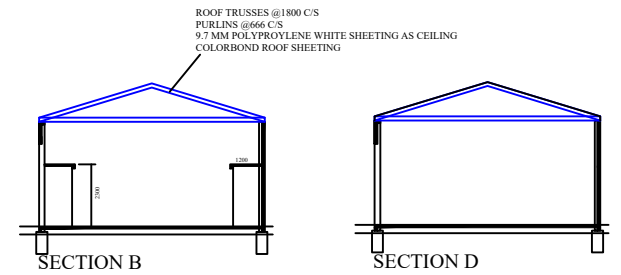
SECTION B
