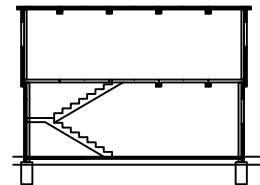
STAIR PROFILE
