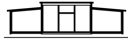
SECTION B STRUCTURE
