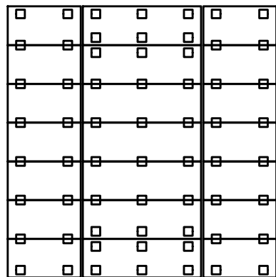
FOOTINGS, FLOOR PANELS
