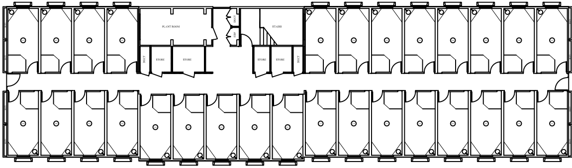
SECOND FLOOR LAYOUT
