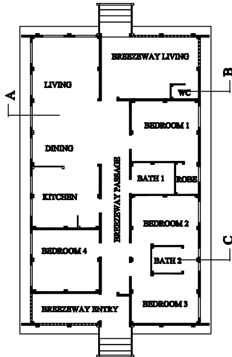
STRUCTURAL UNIBUILD SHELL
