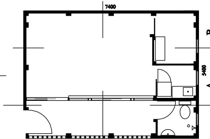
FLOOR PLAN C
