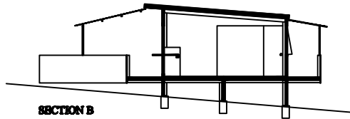
SECTION B
