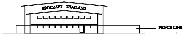
FRONT ELEVATION
