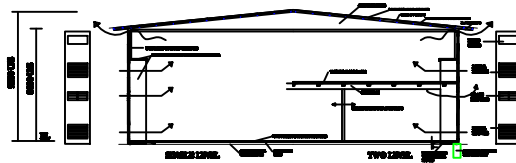
SECTION FACTORY
