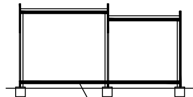
SECTION C
