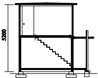
SECTION B
