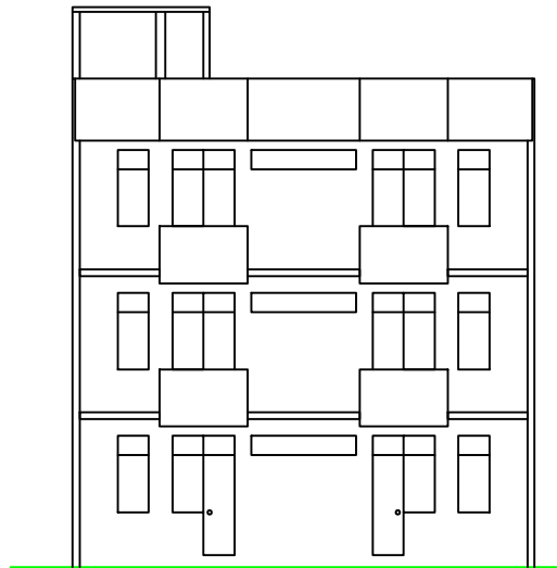
REAR ELEVATION
