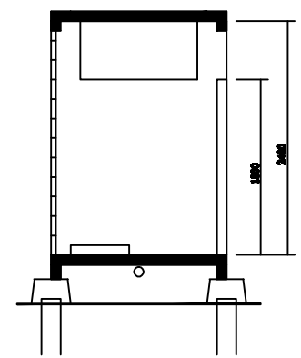
SECTION A
