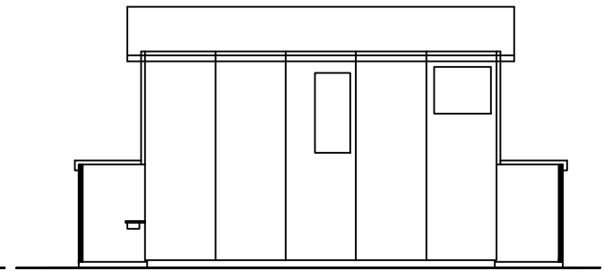
SIDE 4
