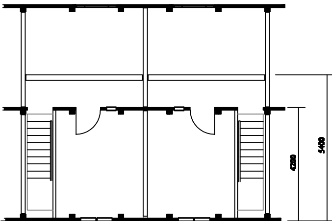
UPPER FLOOR
