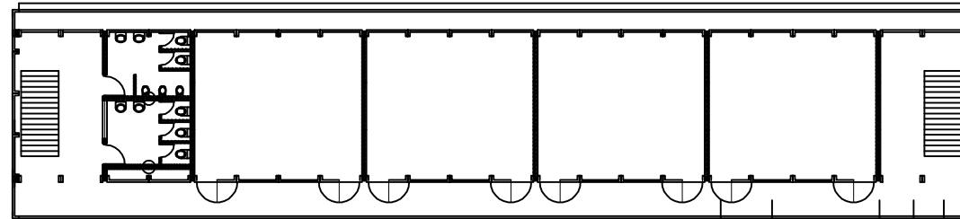
UPPER FLOOR PLAN
