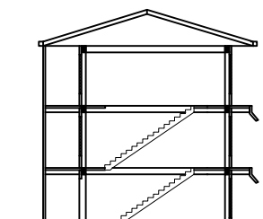
SECTION B
