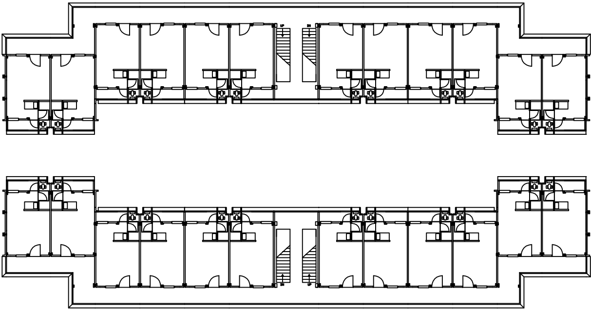
PLAN - FLOORS 1,2,3,4.
