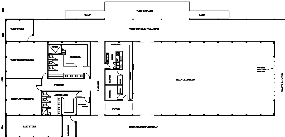
FLOOR PLAN
