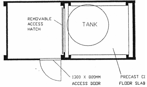
LOWER FLOOR PLAN
